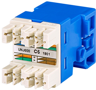
Uniprise Modular Jack, RJ45, category 6, T568A/T568B, unshielded, without dust cover, blue
