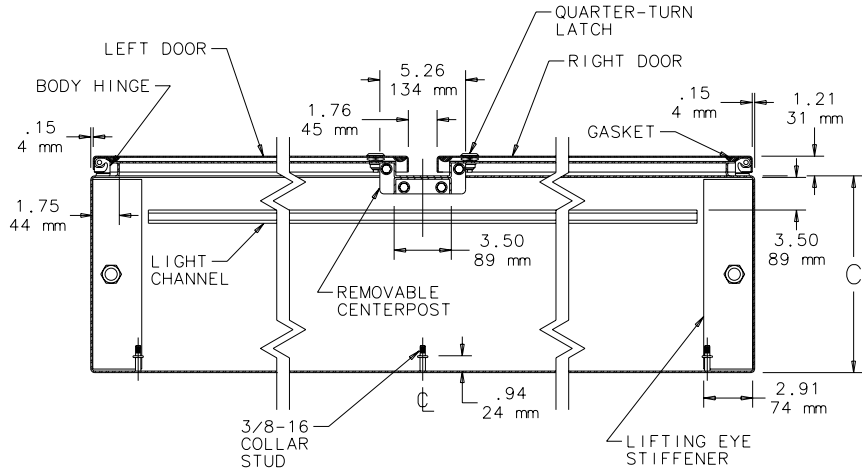
SECTION X-X
