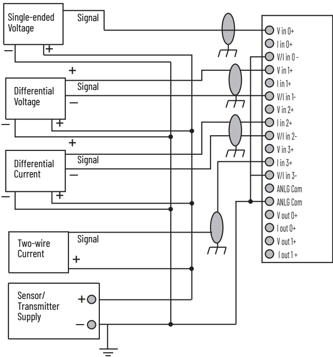
Mixed Transmitter Input Wiring
