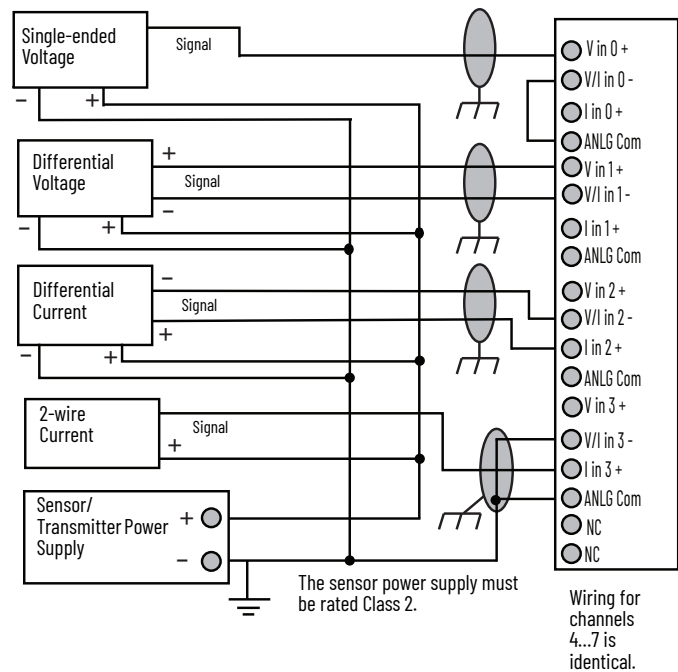
Mixed Transmitter Wiring
