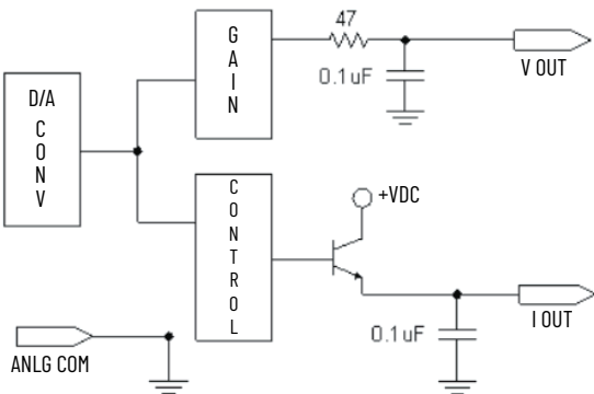
Simplified Output Circuit Diagram
