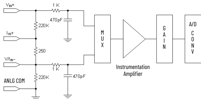
Single-ended Sensor/Transmitter Input Wiring
