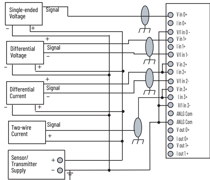
Mixed Transmitter Input Wiring
