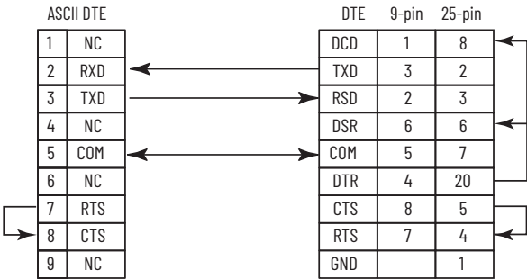
RS-232 Wiring - Module to Printer (hardware handshaking enabled, standard printer adapter cable)
