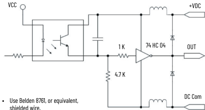
Simplified Output Circuit Diagram
