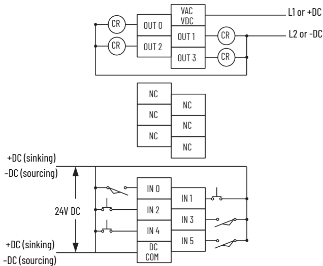
Input and Output Wiring
