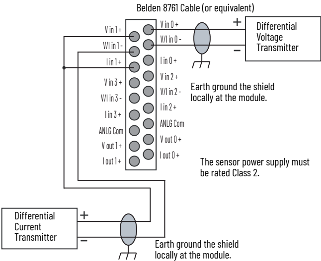
Differential Input Wiring
