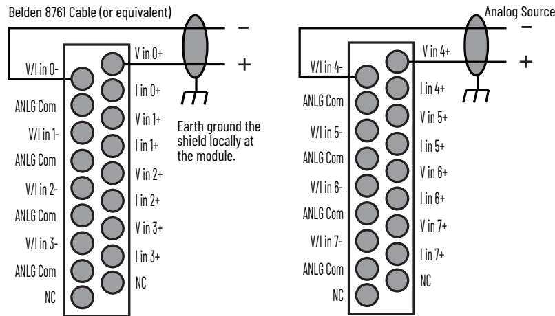
Differential Input Wiring
